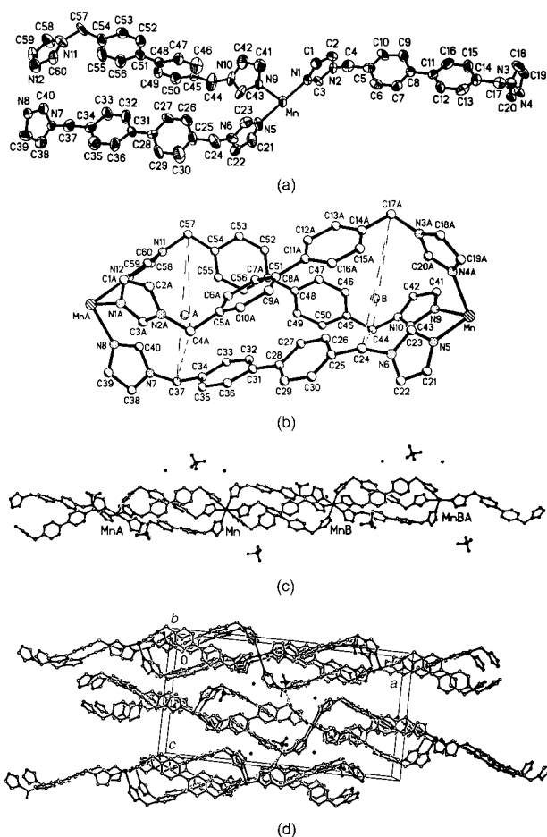
Fig. 1 (a) Crystal structure of the repeat unit of cationic moiety of [\text{Mn}(\text{bimb})_3][\text{ClO}_4]_2\cdot 2\text{H}_2\text{O} with the ellipsoids drawn at the 50% probability level. (b) An individual cage formed by two \text{Mn}^{\text{II}} and three bimb ligands. (c) Poly-cage structure. (d) Crystal packing diagram on the ac plane with hydrogen bonds indicated by dashed lines.
